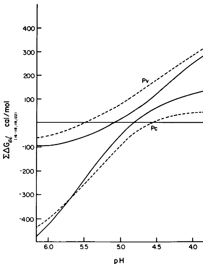
Figure 4 Summed electrostatic free energy between Lys-16 and Arg-118, His-119, and Asp-122, \Sigma\Delta G'_{el} (16-118, 119, 122), in sperm whale myoglobin (Pc) and seal myoglobin (Pv) as a function of pH between 6.0 and 4.0. Computed values at 25°C are shown for I = 0.01 M (—) and I = 0.10 M (---).
