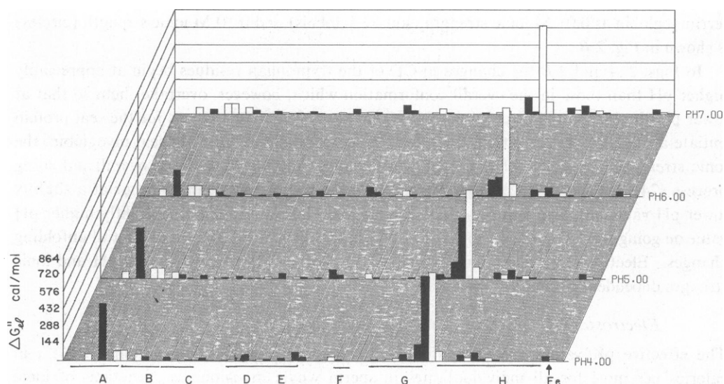
Figure 3 Computed free energy of electrostatic interaction between Lys-16 and each of the other charge sites, \Delta G_e^0 , in calories per mole for sperm whale myoglobin. The diverse charge sites are indicated by their helix references; the iron site is marked on the right hand end and is followed by the propionic acid sites. Negative (stabilizing) free energies are denoted by open bars, and positive (destabilizing) free energies are denoted by solid bars. The results are shown for an ionic strength of 0.01 M and 25°C.
